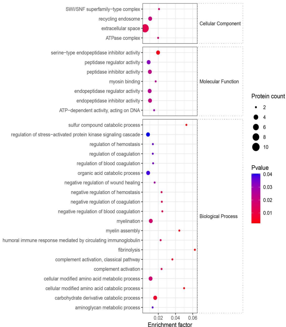
Figure 5 GO enrichment
