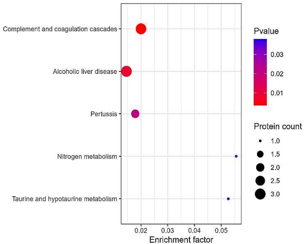
Figure 6 KEGG
