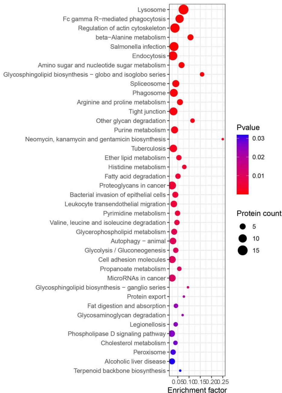
Figure 4 KEGG
